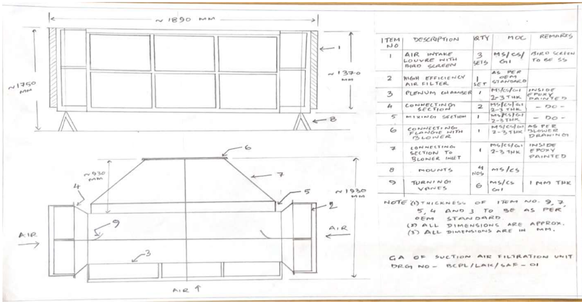
Schematic Drawing Filter SAF-1
