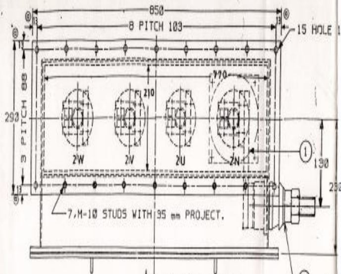
VIEW FROM L.V. SIDE PLAN
