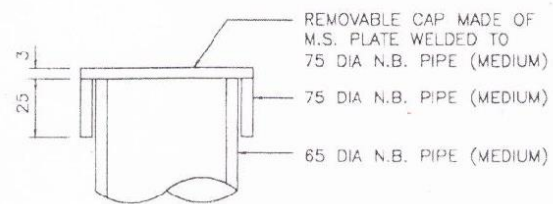
DETAIL-1
