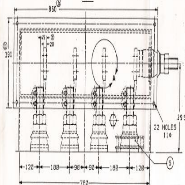
FRONT VIEW FROM LV SIDE
