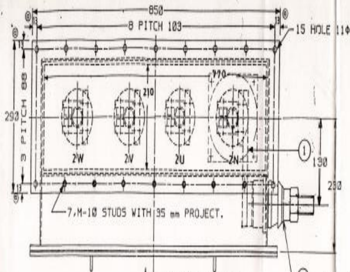
VIEW FROM L.V. SIDE PLAN
