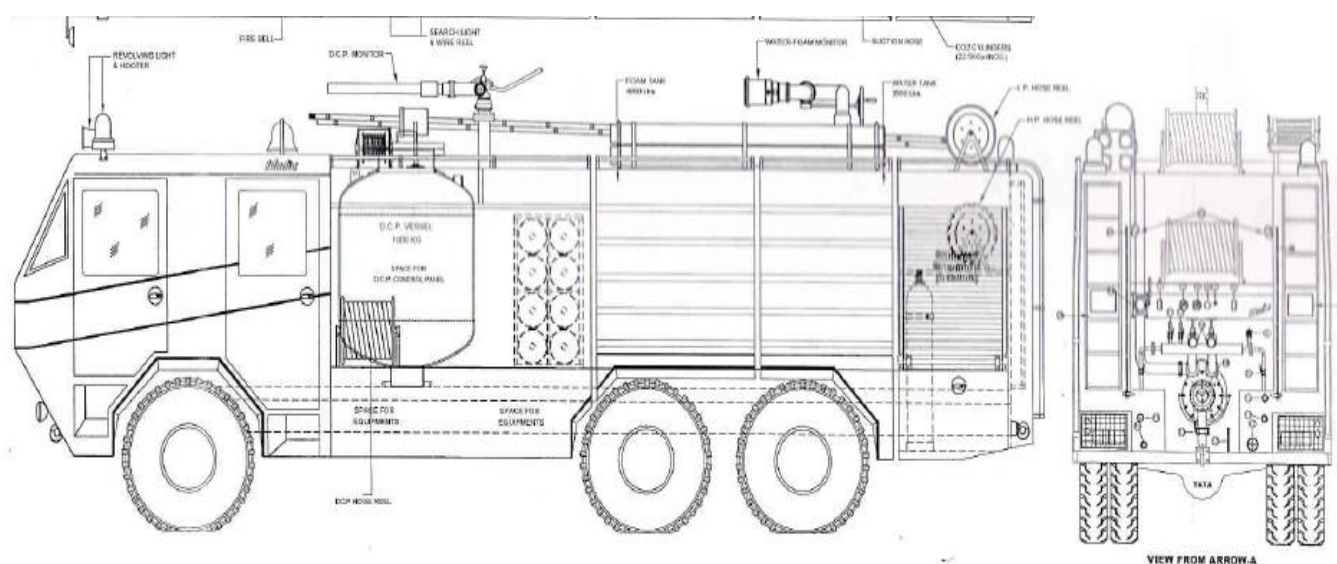
a) Figure 1: INDICATIVE LAYOUT OF DCP CUM FOAM FIRE TENDER ON 28 TON GVW CHASIS
