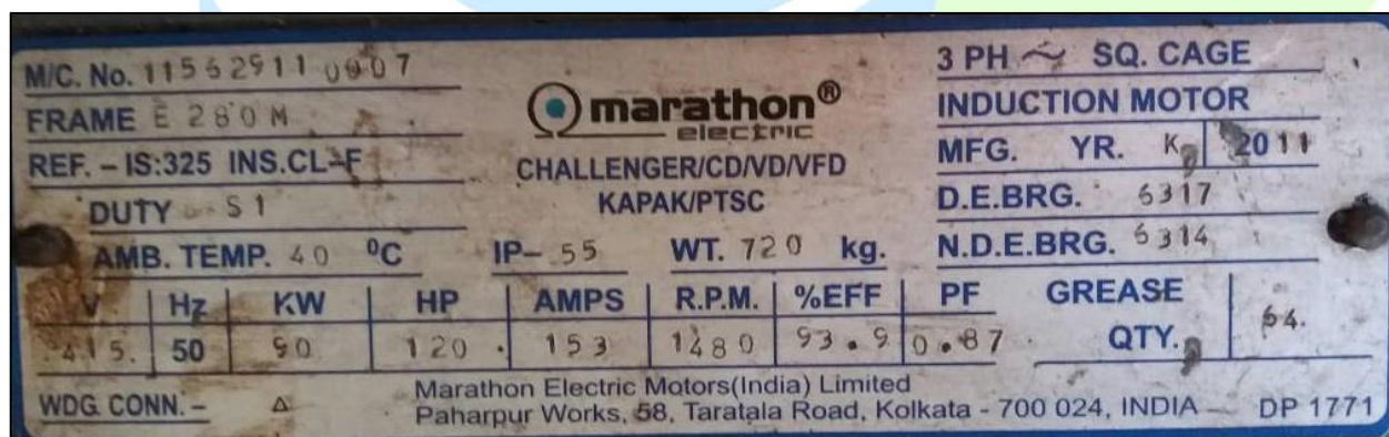
Figure: NAMEPLATE of the existing Motor installed at BCPL Plant.
