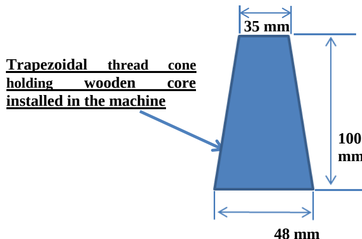
(Top Dia. = 35 mm; Bottom Dia. = 48 mm; Length = 100 mm) (Drawing-2)
