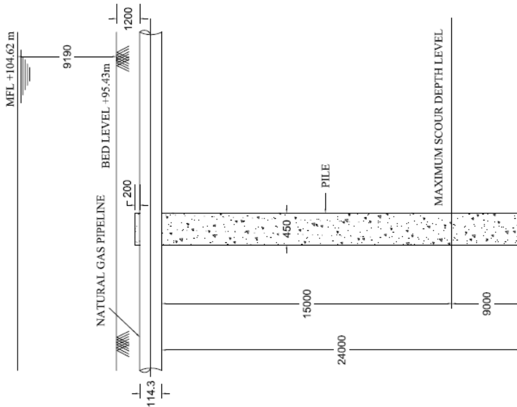
FIXING THE DEPTH OF THE PILE
