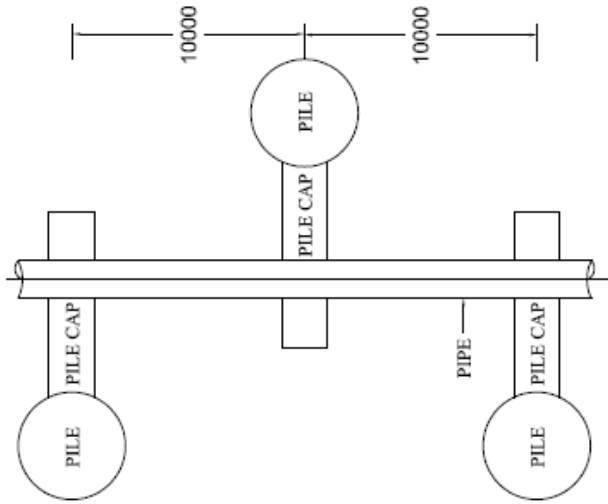
TYPICAL ARRANGEMENT OF PILE - PLAN
