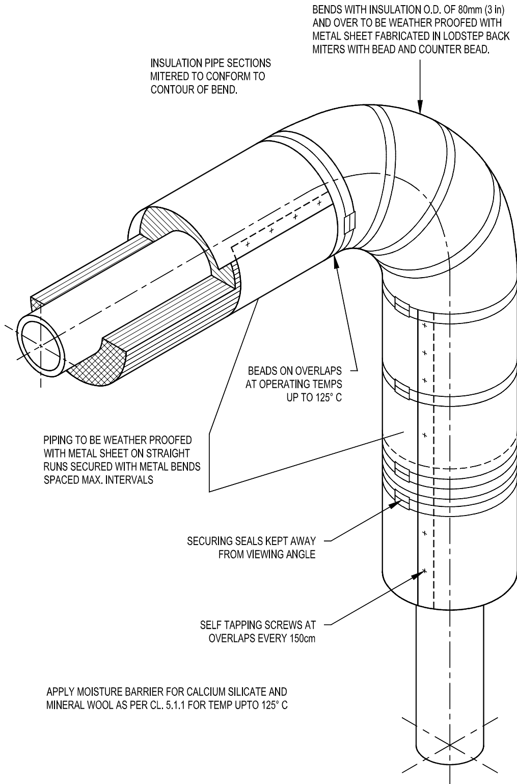
FIGURE – 06 INSULATION DETAILS FOR BENDS / ELBOWS
