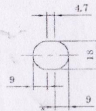
DETAIL OF SLOT
