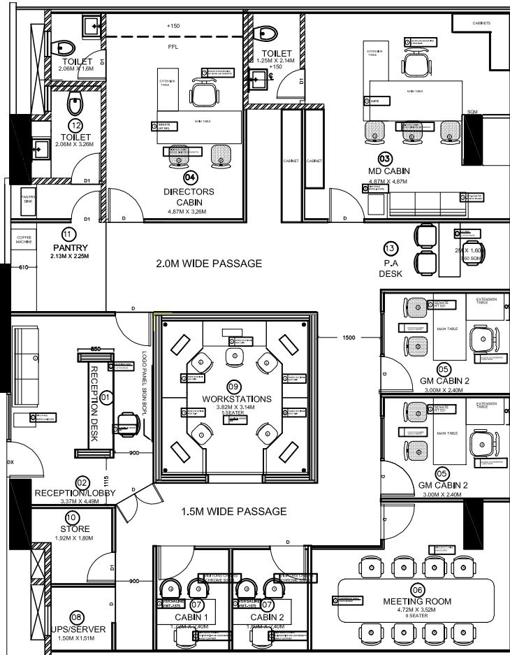
FLOOR PLAN
