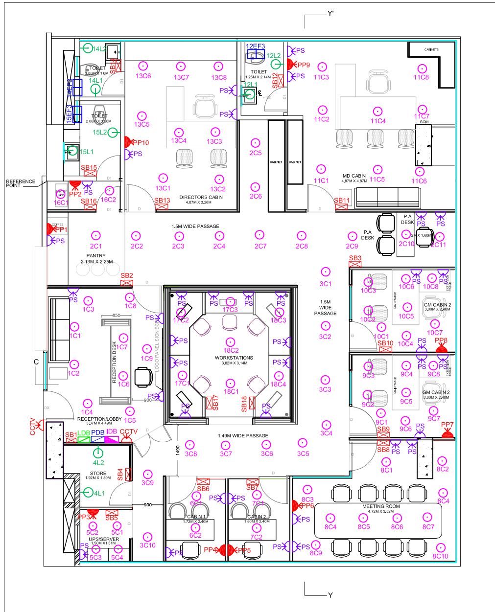
FLOORING PLAN
