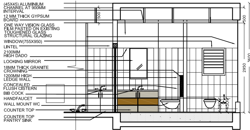
SECTION AT CC'
