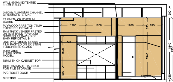
SECTIONAL ELEVATION AT 03/B
