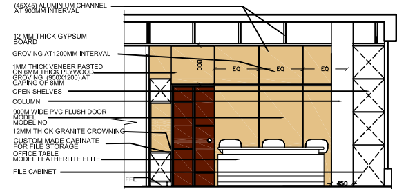
SECTIONAL ELEVATION AT 03/A
