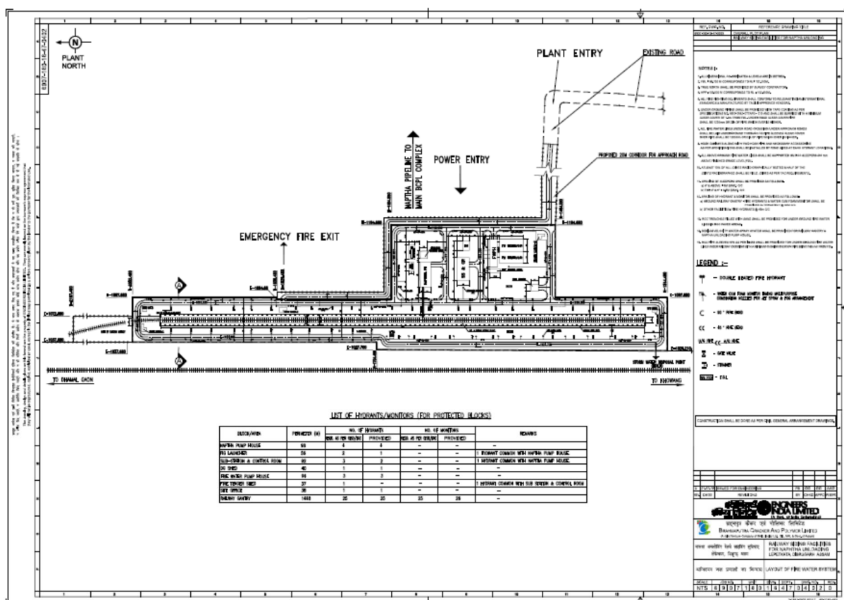
a) Figure 1: 6907-160-16-47-0402-Rev0 Model-LAYOUT FWS-RAILWAY SIDING
