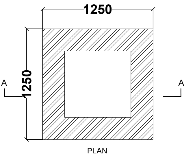
DETAIL OF INSPECTION CHAMBER
