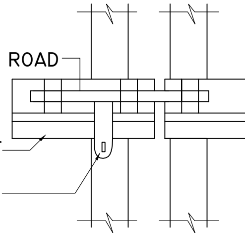
LOCKING ARRANGEMENT AT "L"
