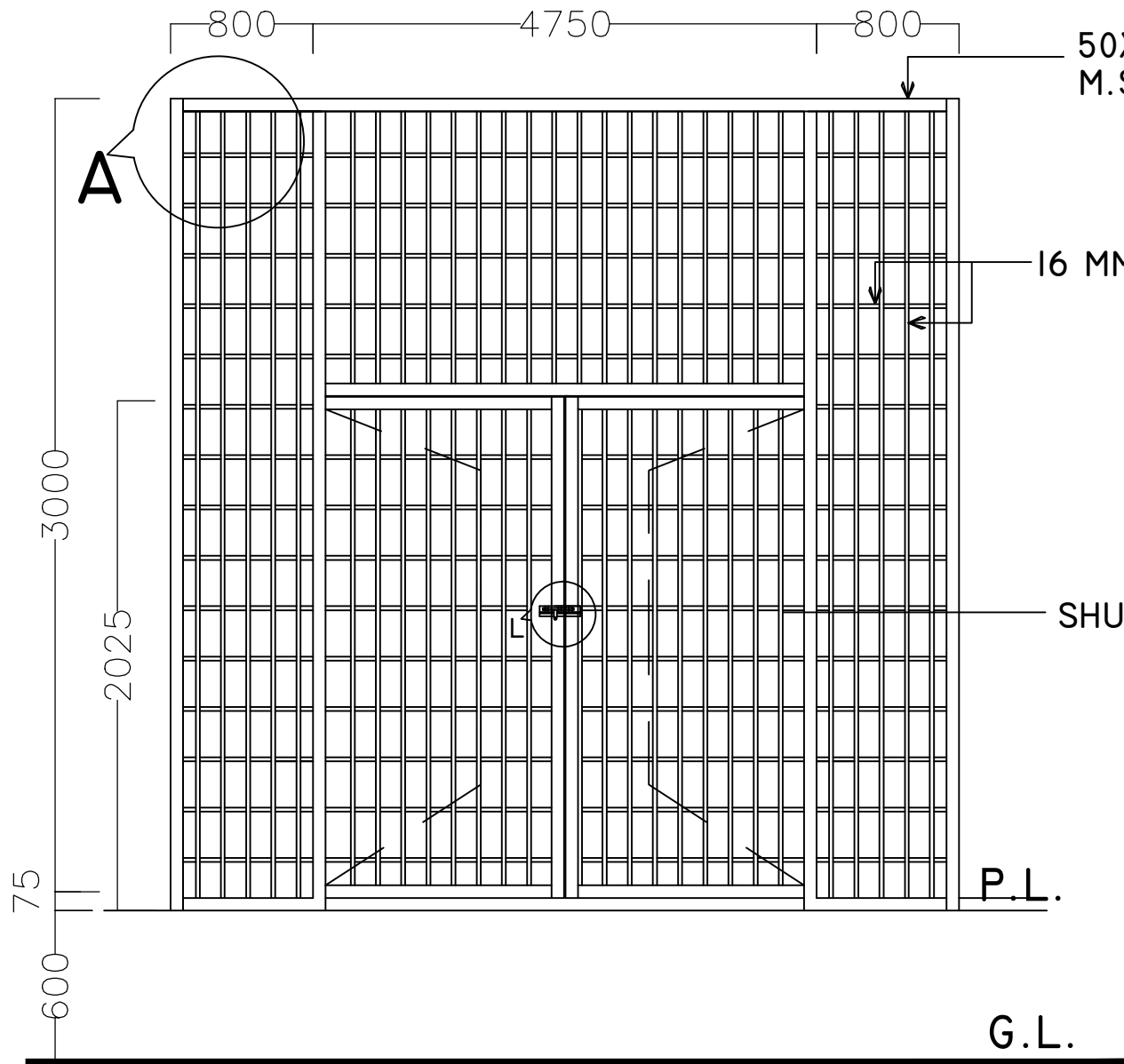
M.S. GRILL WITH M.S. GATE
