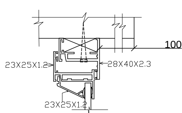
SECTION AT G-G
