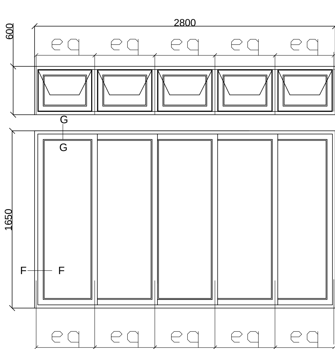
SLIDING WINDOW TYPE- W/V
