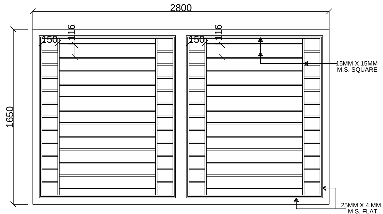
WINDOW GRILL
