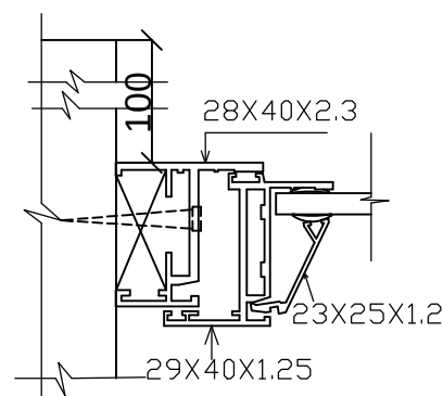
SECTION AT F-F
