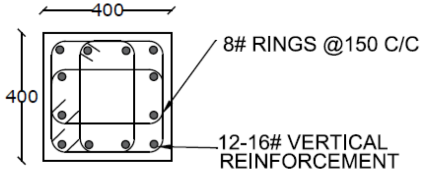
DETAIL OF COLUMN SECTION 2-2
