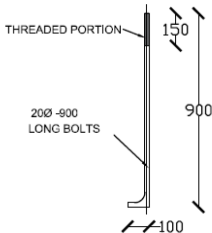
HOLDING DOWN BOLTS MS 20 dia -900 LONG -32 NOS
