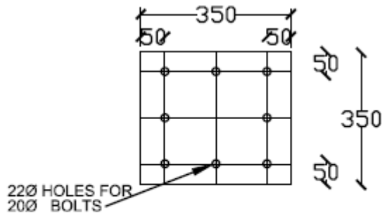
DETAIL OF BASE PLATE 350X350X20 TK.-4 NOS. ( COLUMN C1 TO C4)
