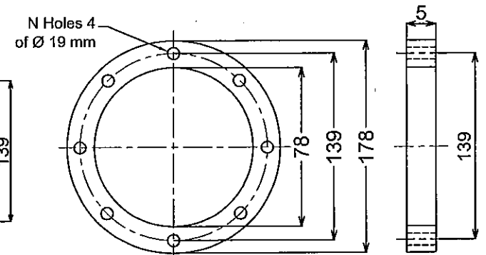
RETAINING RING B FLANGE
