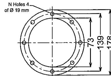
RETAINING RING A FLANGE
