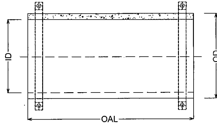
KANWAL RUBBER SLEEVE CONNECTOR (STYLE K-5)
