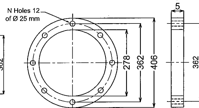
RETAINING RING B FLANGE
