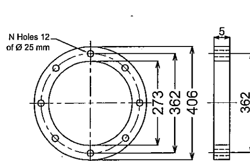
RETAINING RING A FLANGE
