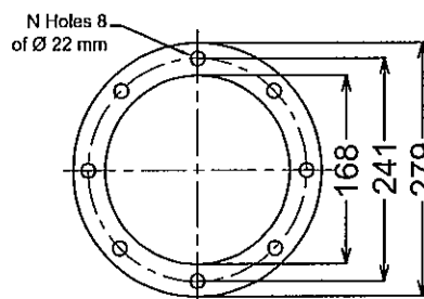
RETAINING RING A FLANGE
