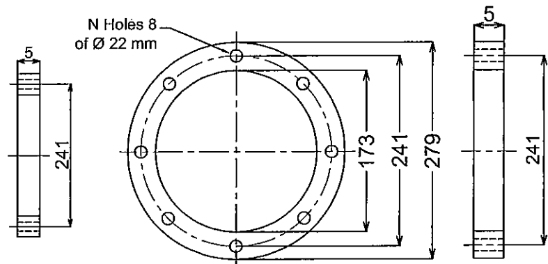
RETAINING RING B FLANGE
